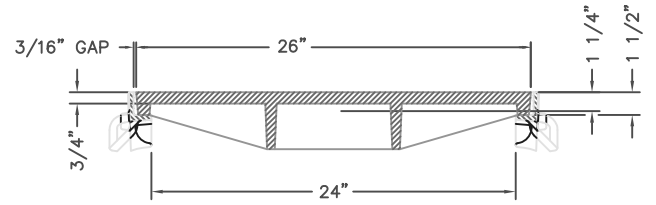
R-4999-HX E TYPE "D" LID w/ TYPE "B" FRAME TYPICAL SECTION THROUGH TRENCH
