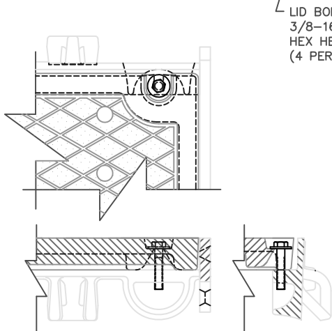
FRAME & LID SHOWING DEBRIS CHUTE SCALE 1:4
